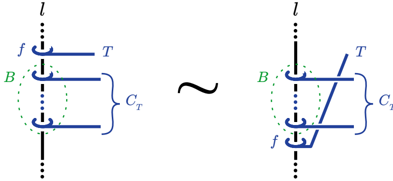
FIGURE 21. Illustration of Lemma 4.5
